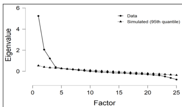
Figure 1 Scree plot of EFA results
