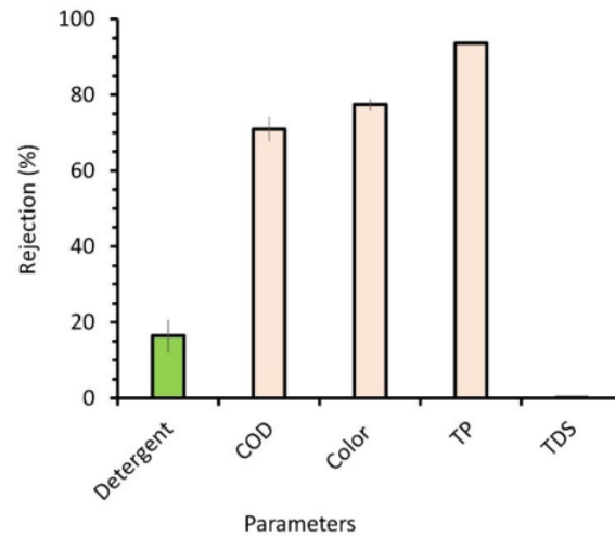
Figure 5. Rejection performance of laundry wastewater filtration.
