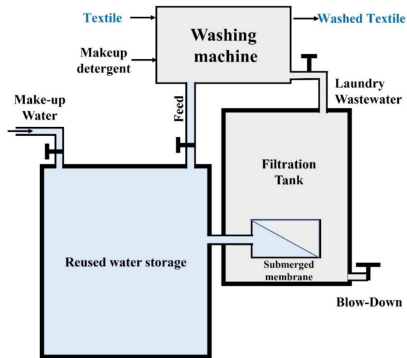
Figure 6. Practical implementation of reuse of laundry wastewater for laundry services.
