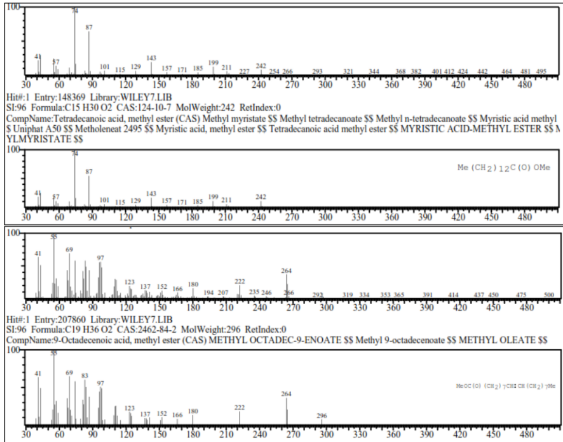
Figure 2. Spectrum of used cooking oil biodiesel components
