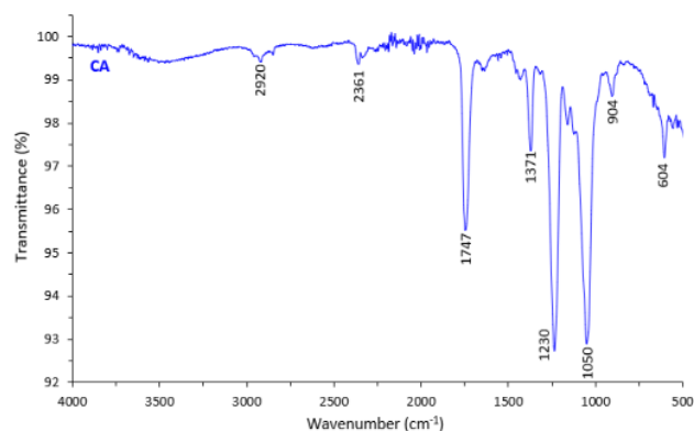
Figure 6. FT-IR spectra of the cellulose acetate membrane.
